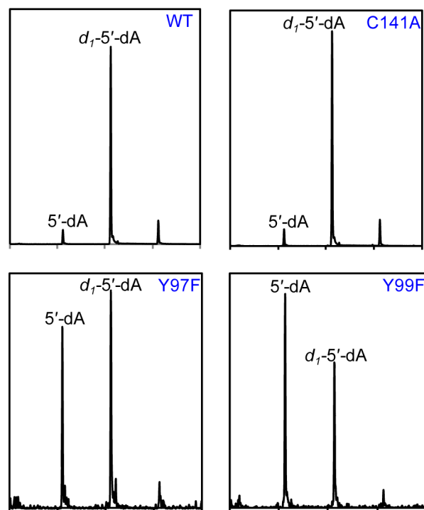
Figure 4. Mass spectrometry analysis of 5'-dA isolated from Bs SPL reactions conducted with d 1 -SP TpT as the substrate. d 1 -5'-dA forms via abstraction of a H atom from d 1 -SP TpT, and the unlabeled 5'-dA forms via uncoupled SAM cleavage. The exact mass for each 5'-dA species is given in the Supporting Information.
